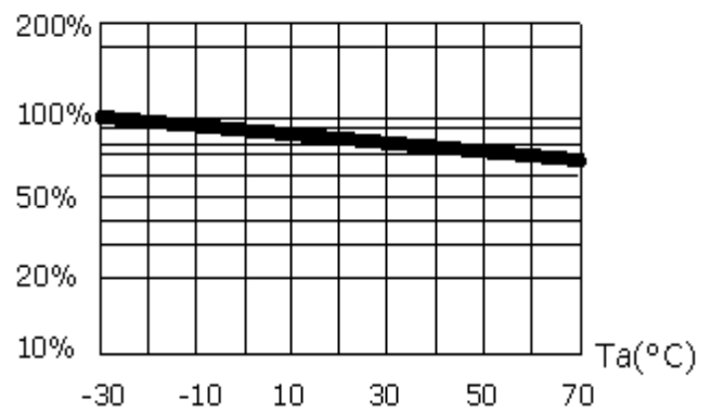
Fig. 5 Relative Luminous Flux vs Ambient Temperature
