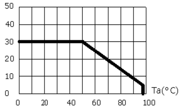
Fig. 3 Maximum Forward Current vs Ambient Temperature
