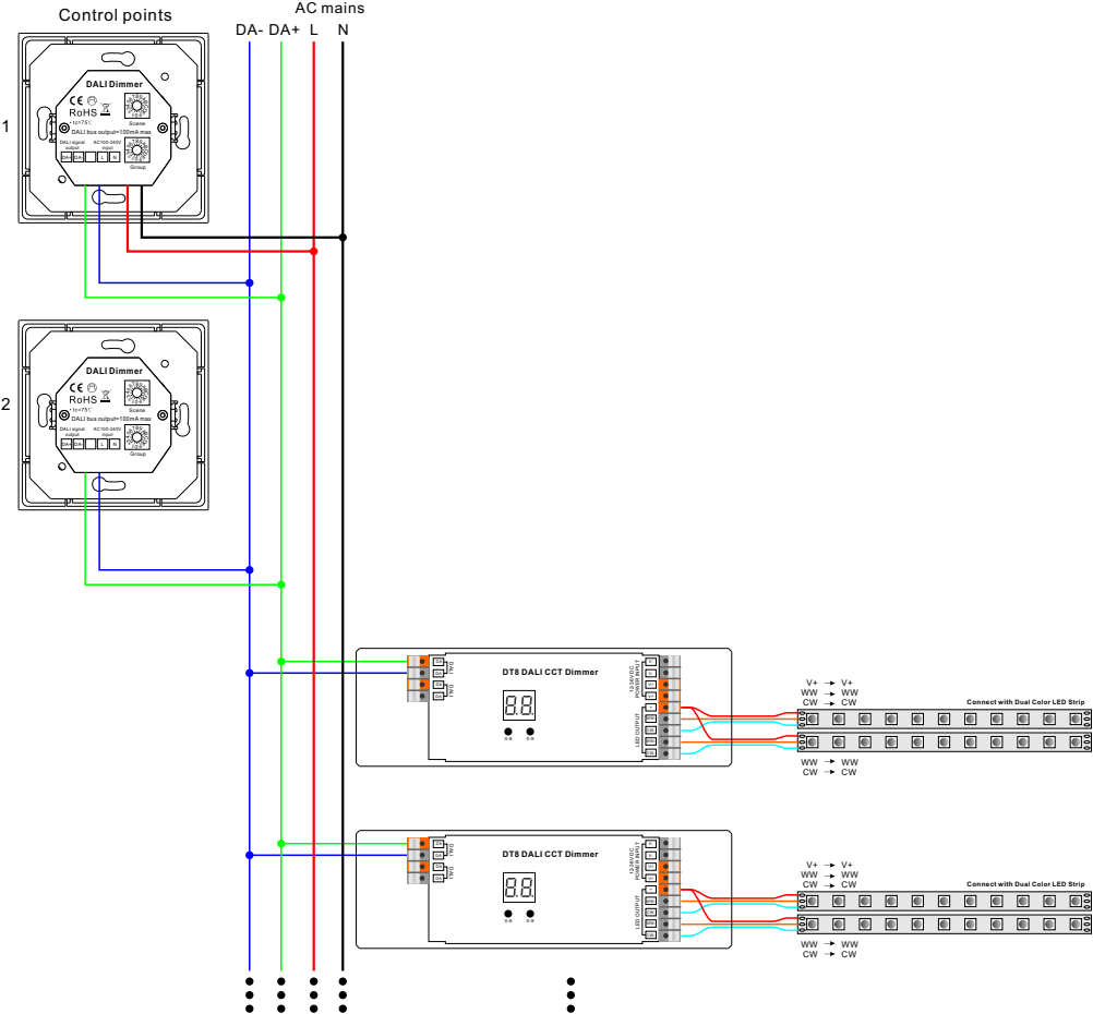
Figure 2: Supply DALI bus power to the DALI system and add the device into the DALI system
