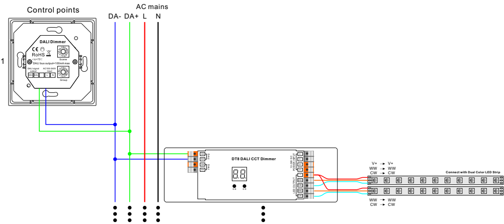
Figure 2: Supply DALI bus power to the DALI system and add the device into the DALI system
